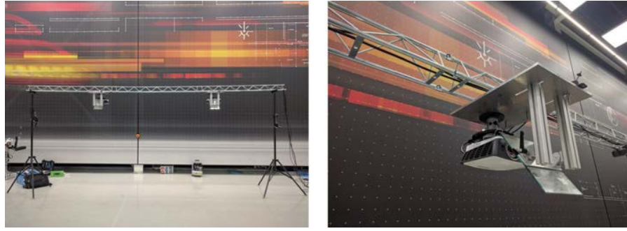
Figure 8.8: Implementation of the floor projection system. (left) Two projectors on trussing (right) close view of projectors with front-facing mirror
