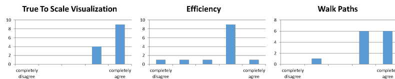
Figure 8.11: Survey results on: original size visualization (left), efficiency improvements (middle) and verification of walking paths (right) (compare Otto et al. [93])
