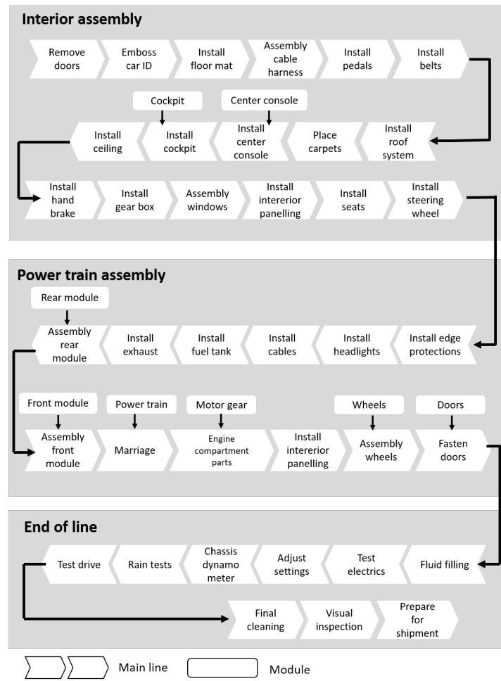
Figure 3.6: Generalized structure of automotive final assembly work contents (based on Weyand [48])
