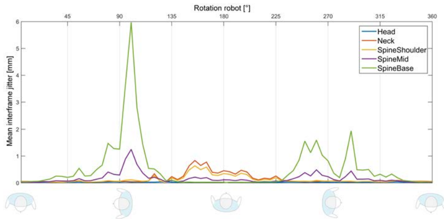
Figure 7.7: 360° experiment: Mean inter-frame jitter for all center-axis joints [174]
