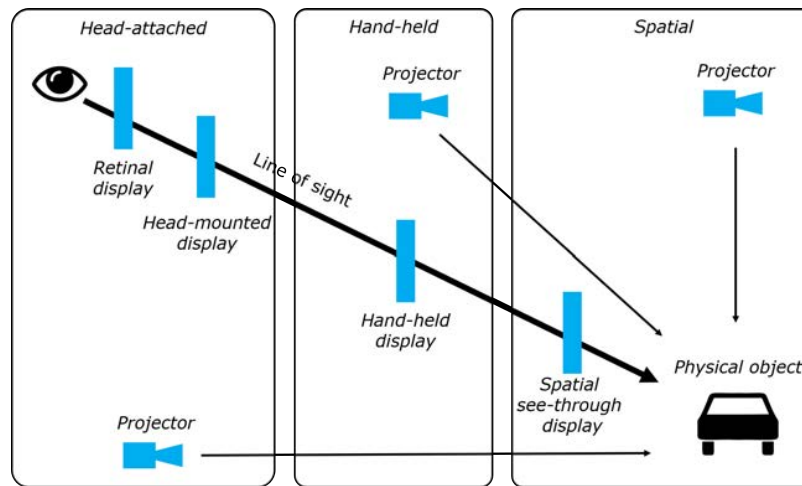
Figure 9.1: Visual display techniques and positioning (based on Bimber and Raskar [287])
