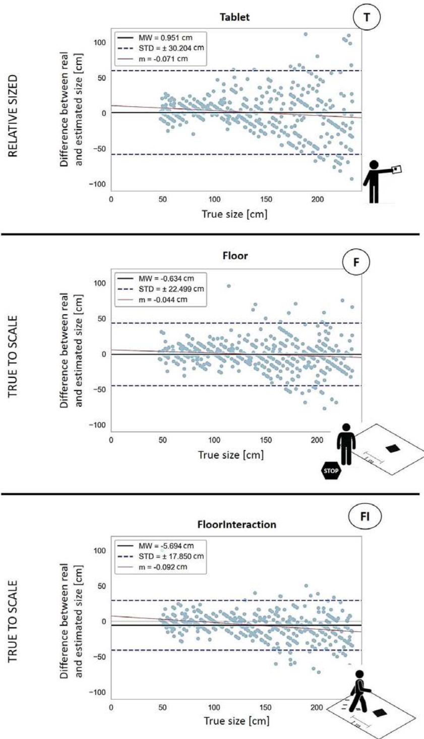
Figure 8.17: Scatter plots of all three scenarios show the spatial deviations. Each plot follows Bland-Altman plot [282] style, additionally showing the mean values, standard deviations and a linear regressions over the actual visualized cube sizes. One can see that variance of spatial deviations over the true sizes tends to increase in all scenarios [239, 245]
