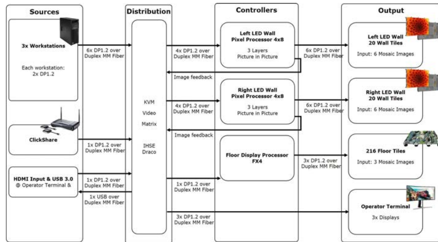
Figure 8.13: System architecture of the VMS image distribution and controllers to the devices
