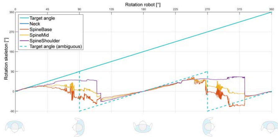
Figure 7.6: 360° rotational experiment: Expected SDK behavior vs. estimated shoulder and hip orientation [174]
