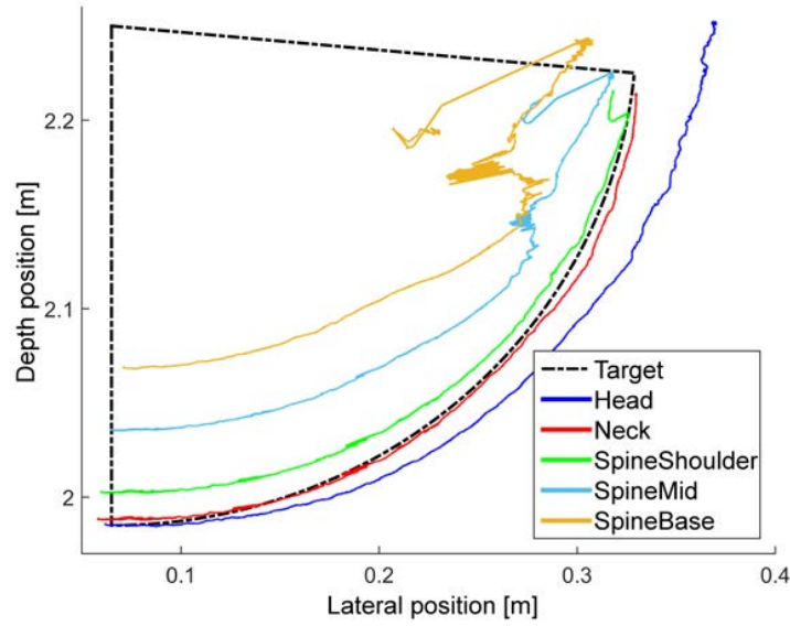
Figure 7.8: Evaluation of 85° experiment: top view of center-axis joints in relation to ground truth real trajectory [174]
