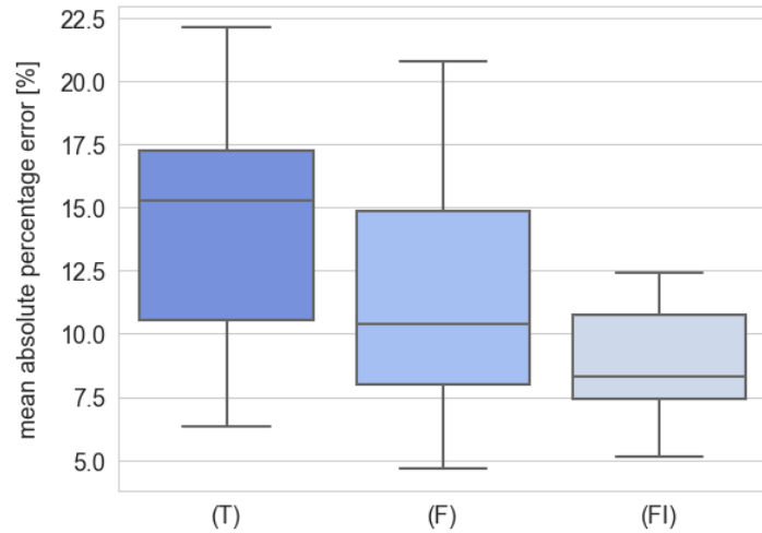
Figure 8.18: Box plot for MAPE of scenarios (T), (F) and (FI) [239, 245]
