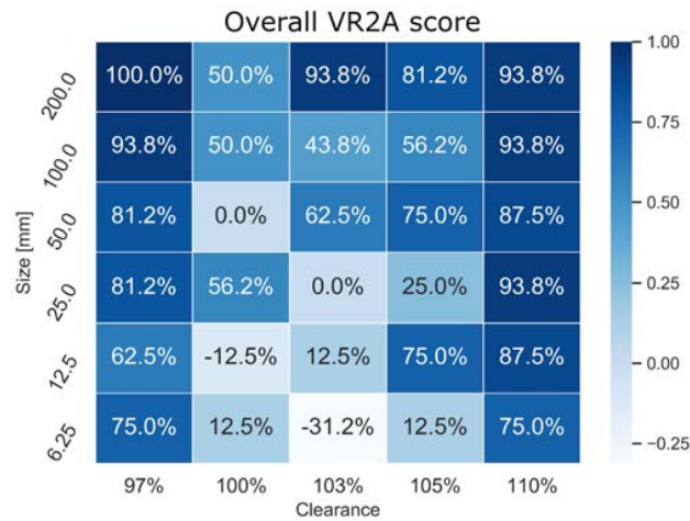
Figure 6.14: Results of the VR assembly assessment score. Low values indicate high uncertainty or inhomogeneity of answers [124]
