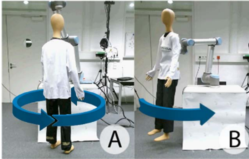
Figure 7.3: Experimental setups: A) 360° rotational test: Mannequin hanging on robot, B) Mannequin's spine mounted on robot [174]
