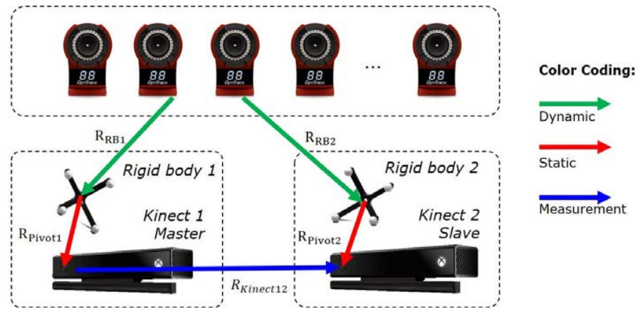
Figure 7.13: Experimental setup for evaluation of Multi-Kinect tracking accuracy
