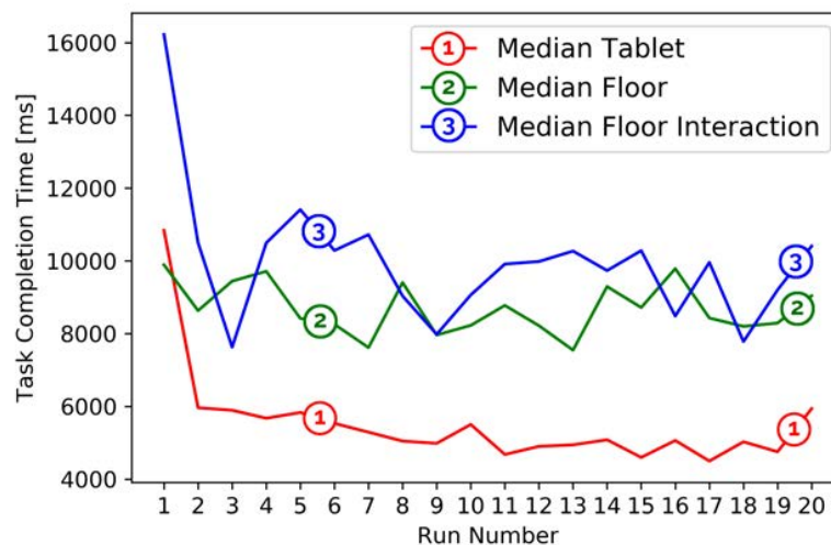
Figure 8.20: Median task completion time of all participants (N=22) for all 3 scenarios throughout the 20 runs [239]
