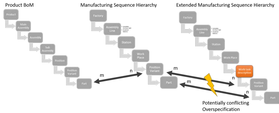
Figure 6.4: Interconnection between product BOM, manufacturing sequence hierarchy and work task descriptions
