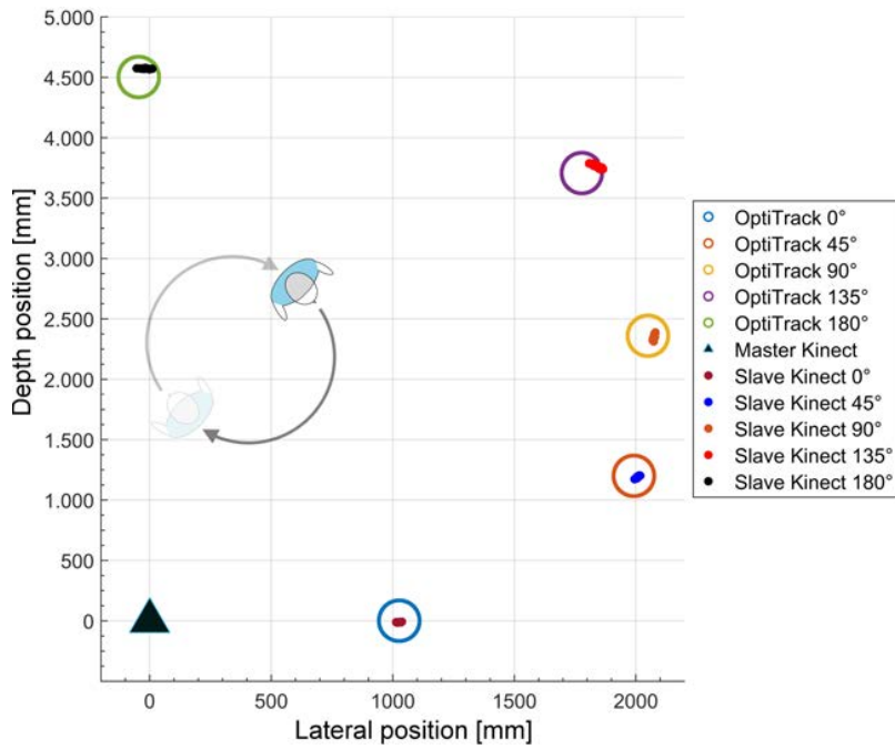
Figure 7.14: Top view of the registration results: Master sensor at [0,0], 5 scenarios with 20 registrations each, circles indicate the ground truth of the OptiTrack measurements [174, 175]
