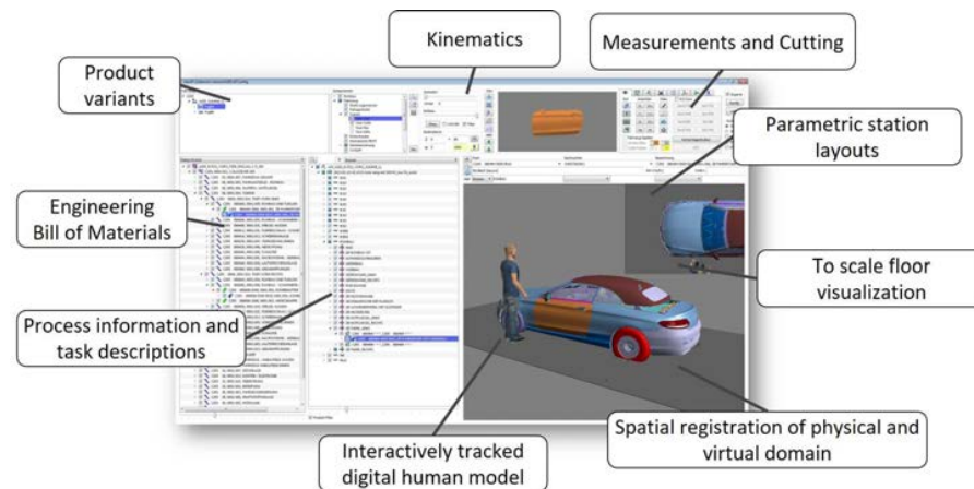
Figure 6.1: User interface of the assembly simulation software veo. (Left) Product variants, manufacturing sequence and eBOM can be switched. (right) 3D visualization of the virtual scene and bird's eye view of the parametric cell layout. (upper right) Manipulating the interactive assembly simulation. (top) Active single part visualization
