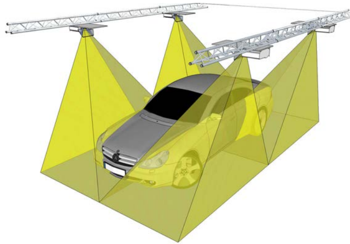
Figure 8.6: Hardware arrangement of floor projection with light paths and projection cones
