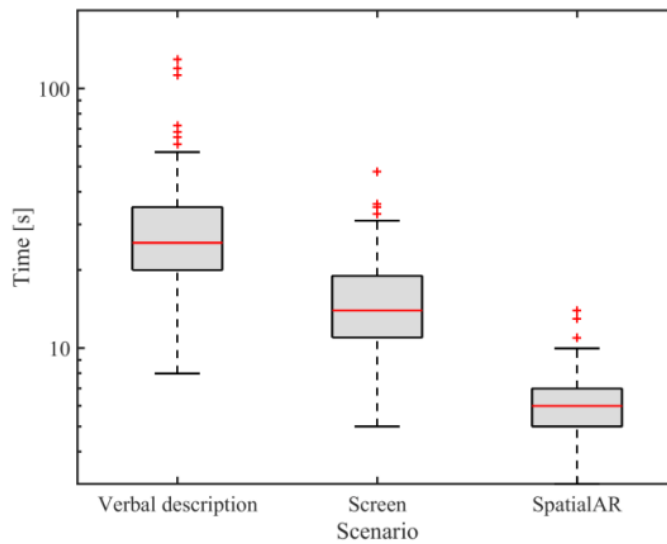
Figure 9.13: Evaluation on mean times and standard deviations (sorted by descending verbal description results) [79]
