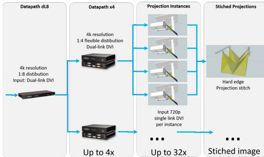
Figure 8.7: System architecture of floor projection system (based on Otto et al. [93])
