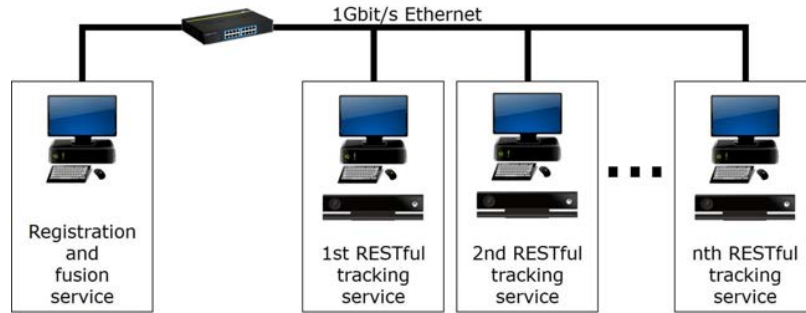
Figure 7.9: Hardware setup for the tracking system with service-oriented, distributed sensor services (based on [174, 175])
