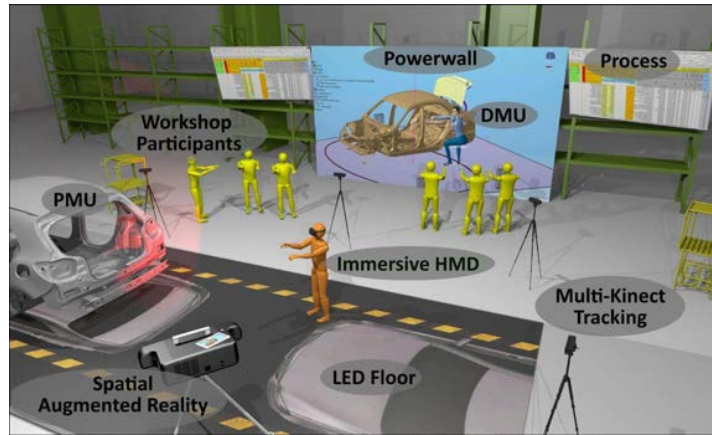
Figure 5.5: Rendering of the vision for an integrated virtual manufacturing station environment as a collaborative workshop environment for interactive assessments of manual assembly tasks [94]
