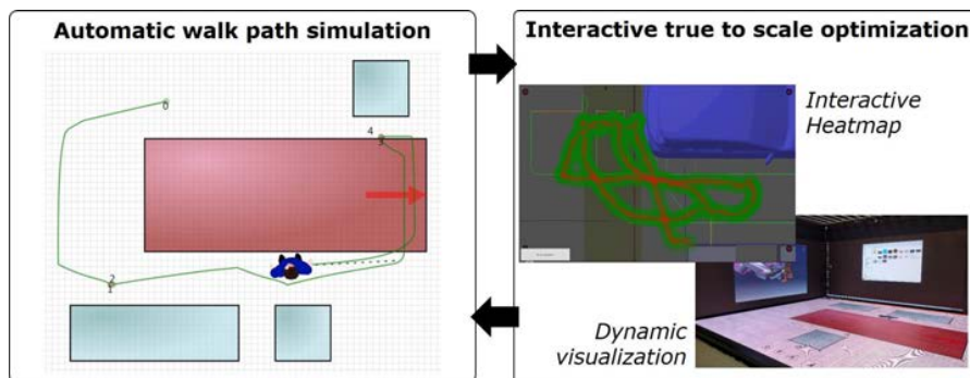
Figure 8.1: Walk path optimizations on the augmented floor surface. A combination of automatically simulated walk paths and interactively recorded walk paths are shown in original size (based on [239])
