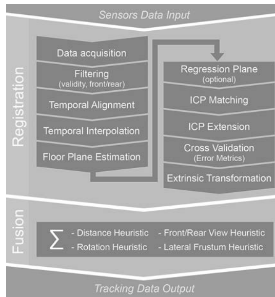
Figure 7.10: Block diagram of fusion service [174, 175]
