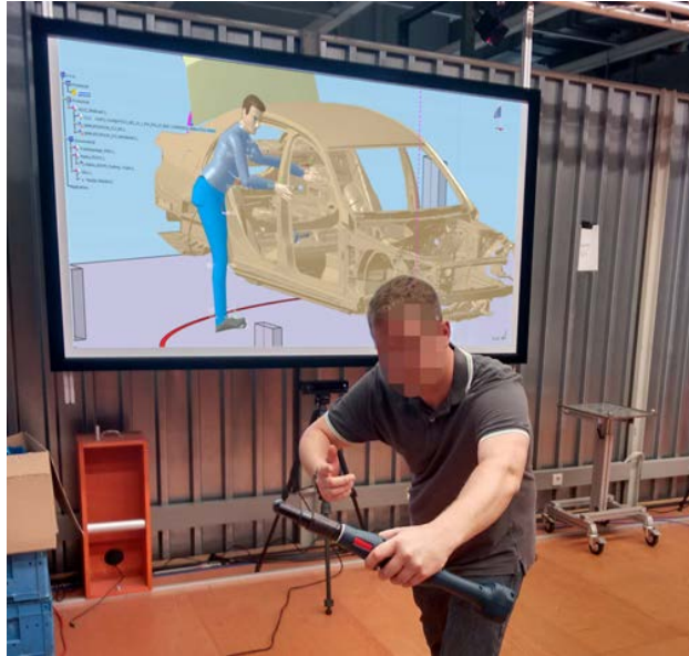
Figure 7.16: Delmia V5 DHM directly manipulated by marker-less motion capture approach. All assessments can be carried out in real time [174, 175]
