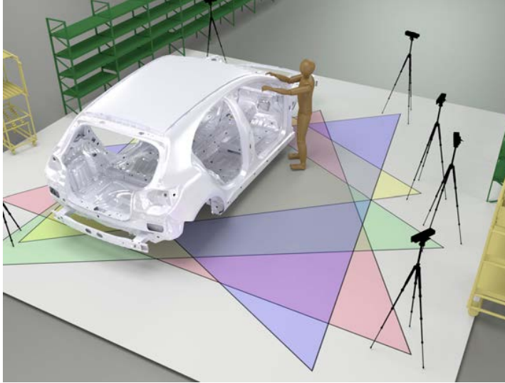
Figure 7.1: Workshop area in automotive car assembly with full body skeletal tracking, typically sized 6m x 4m. This also represents the required tracking area [94, 174]
