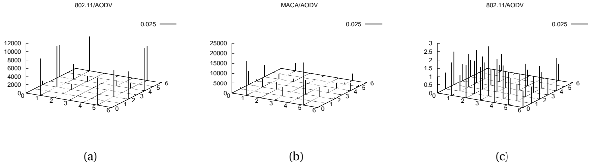
Figure 6.4: Figure showing the spatial distribution of the control overhead for Example 2. The network is as shown in Figure 6.2(b). All the plots are for injection rate of 0.025 seconds. (a) Left: Results for MAC layer overhead for (802.11, AODV). (b) Center: Results for MAC layer overhead for (MACA, AODV) combination. Although the number of MAC overhead packets appears low, it is because the percentage of packets delivered using this combination is substantially lower than what is delivered using (802.11, AODV) combination. (c) Right: Results for Routing layer overhead for (802.11, AODV) combination. The number of control packets was computed as average number of control packets emitted by a given node over 10 simulation runs, i.e. in case of MAC layer control packets it was a sum of RTS, CTS and ACK packets, and in case of routing layer control packets it was a sum of RREQ, RREP packets.
