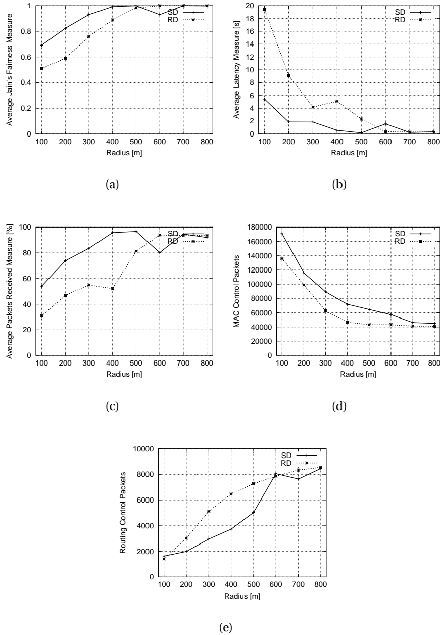
Figure 7.3: (a) A comparison of the Jain's fairness measure, (b) A comparison of the latency measure, (c) A comparison of the average number of packets received (d) The number of control packets for MAC layer, (e) The number of control packets for Routing layer
